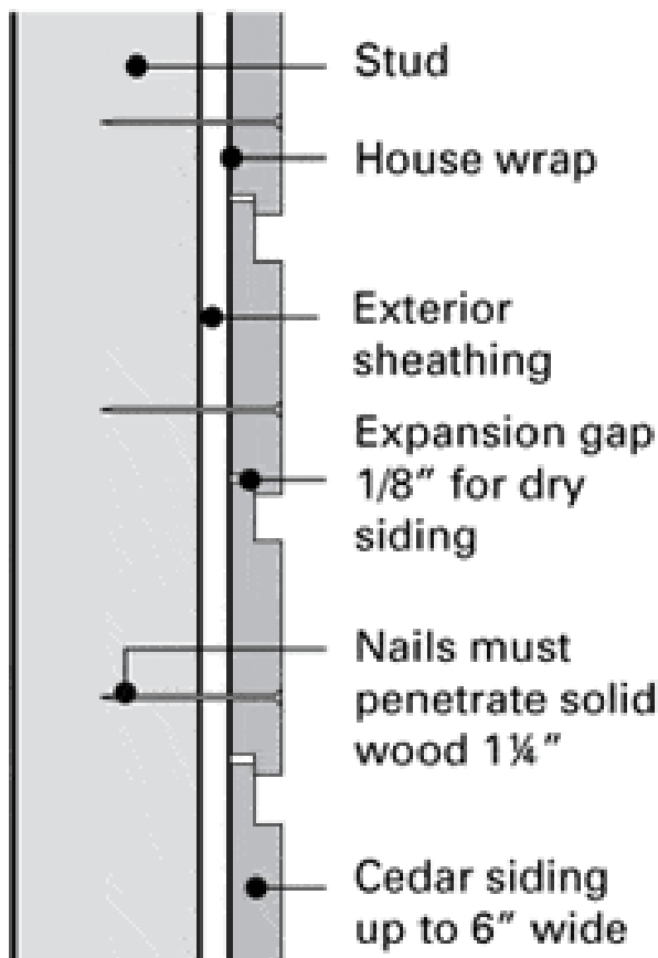
(A) 6" and narrower lap siding
