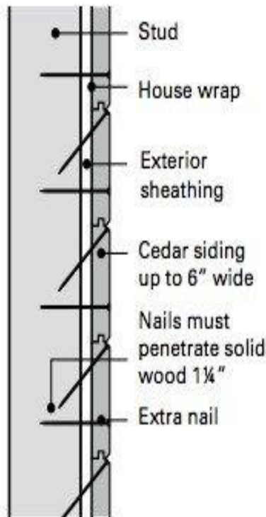
(B) 6" and narrower siding in hot, dry, windy or seacoast climates
