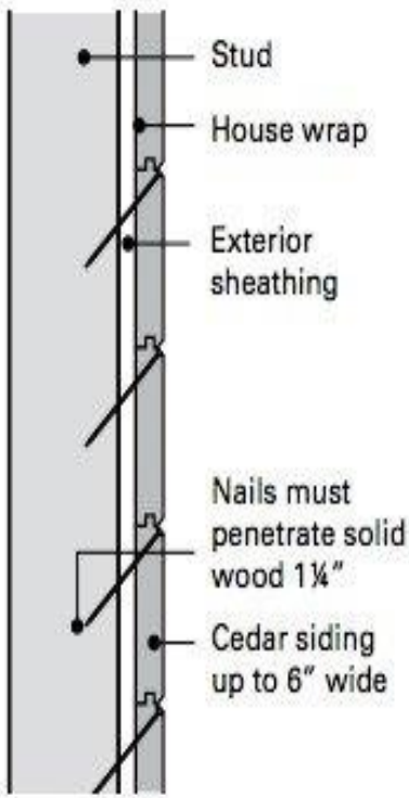
(A) 6" and narrower siding in normal climatic conditions
