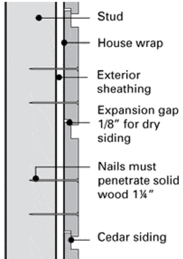
(B) 8" and wider lap siding
